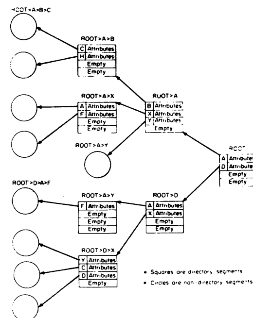
Fig. 4. Directory hierarchy.
