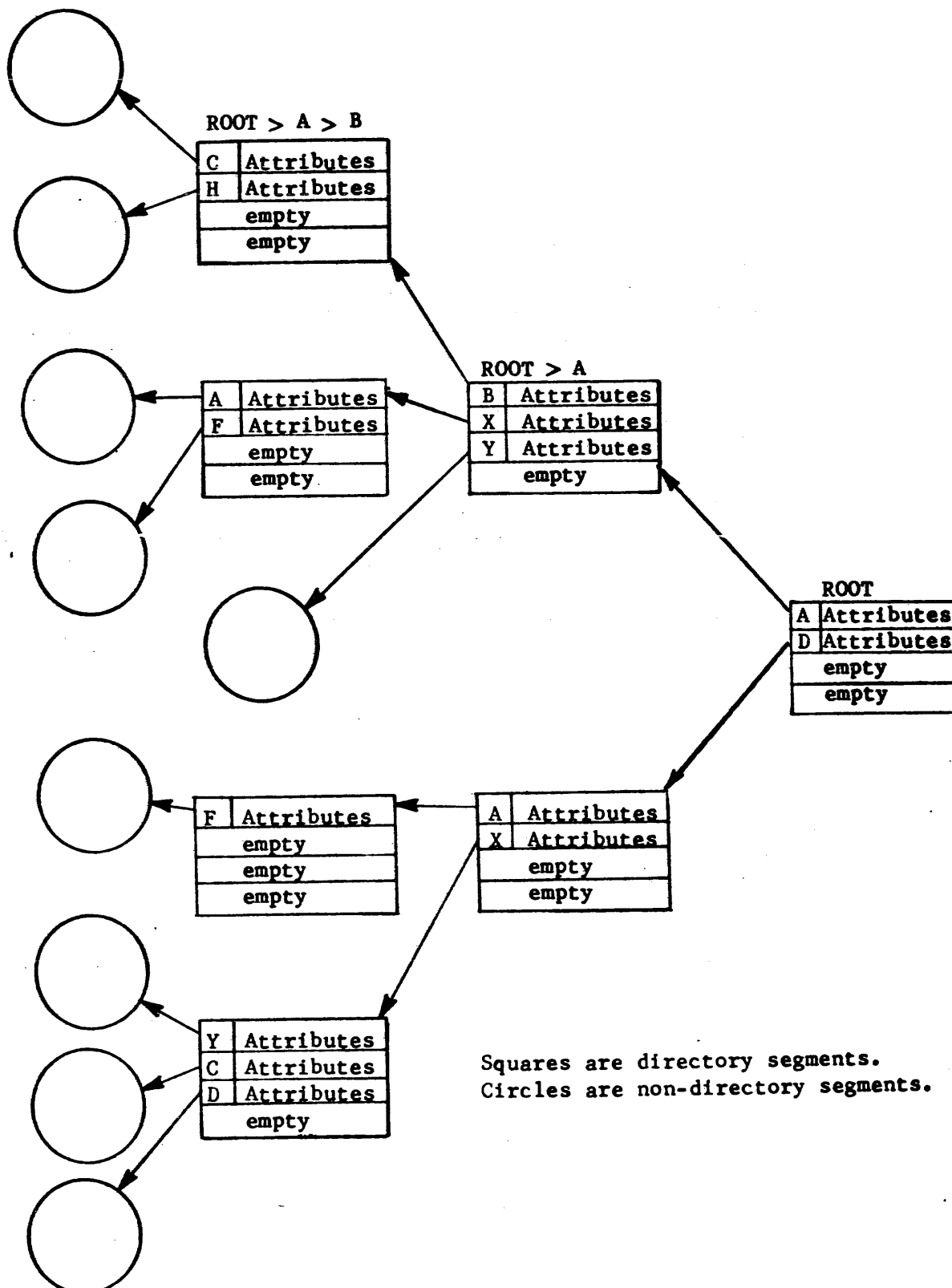
Figure 4. Directory Hierarchy
